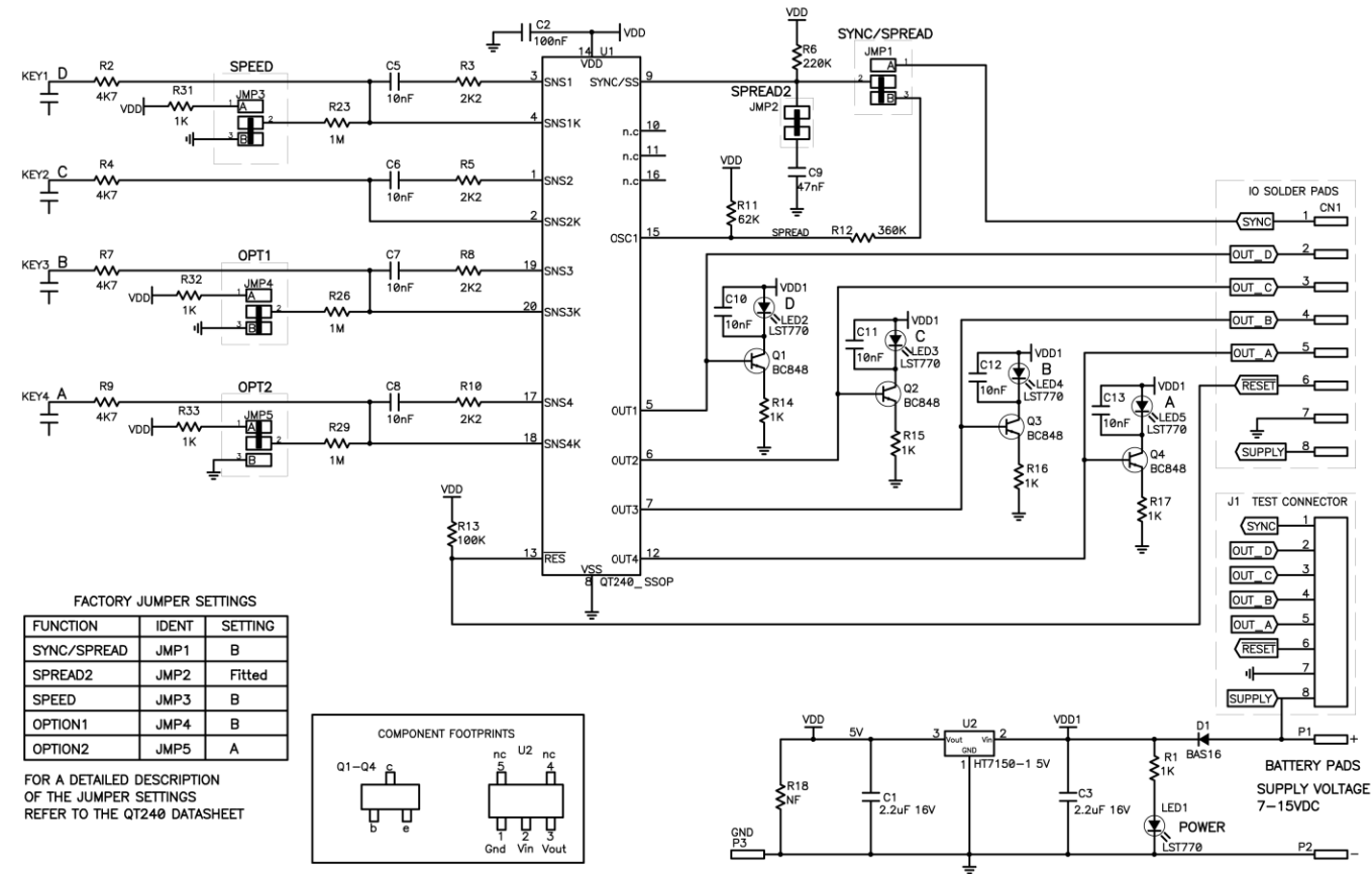
Figure 2 — Schematic Diagram
